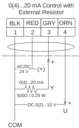
Figure 19: Control Wiring Diagrams
