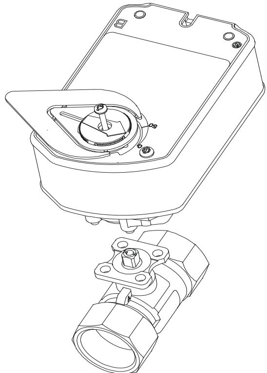
Figure 15: Mount the Actuator
