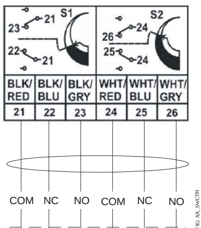
Figure 21: Optional Auxiliary Switch
